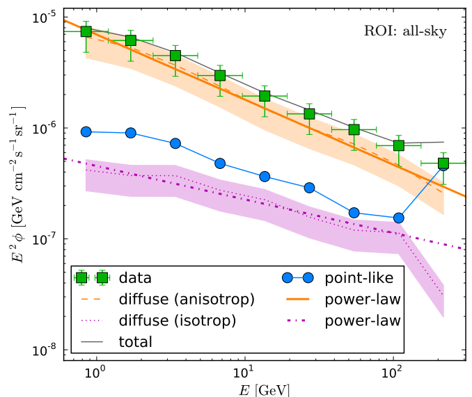
Fig. 4. Illustration of energy spectra considering an all-sky ROI. Shown are the data (green squares) converted to flux units, and spectra from the reconstructed total (gray), anisotropic diffuse (dashed orange), isotropic diffuse (dotted magenta), and point-like photon flux (blue circles). Furthermore, power-law fits for the anisotropic (thick solid orange) and isotropic emission (thick dash-dotted magenta) are shown. The errors include statistical and systematic uncertainties and are only shown for data and diffuse contributions for reasons of clarity.
