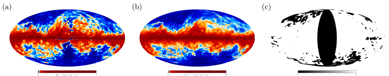
Fig. 8. Illustration of the brightness in Mollweide view. Panel (a) shows the integrated brightness of the “cloud”-like component. Panel (b) shows the monochromatic brightness of thermal dust emission at 353 GHz (Planck Collaboration 2013a). Panel (c) shows in white the area included in computing the latitude profile in Fig. 9.
